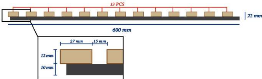
DAKUC-000 2800x600x22mm
